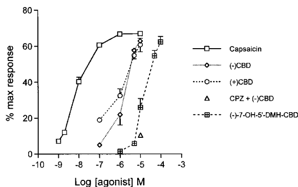
Figure 2 Effect of (-)-CBD, (+)-CBD, (-)-7-OH-5'-DMH-CBD and capsaicin on cytosolic Ca 2+ concentration in HEK-hVR1 cells. The effect is expressed as per cent of the effect of 4 \mu M ionomycin, and data represent means ± s.d. of n=4 experiments. The effect of capsazepine (CPZ, 10 \mu M) on 10 \mu M CBD is also shown (open triangle).
